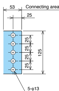
Main circuit terminal dimension
