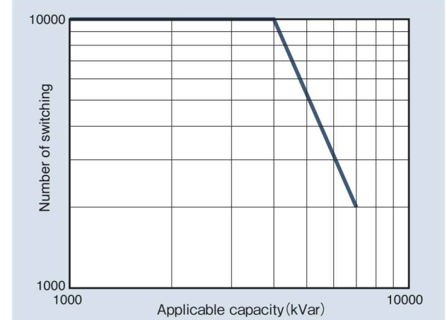
Fig. 107 Guidelines on the switching times for applicable capacity (for 12, 15kV).
