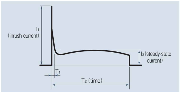
Fig. 102 Motor operation current waveform.
