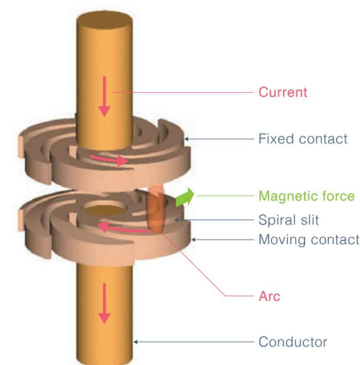
Fig. 3 Current flow at the time of breaking.
