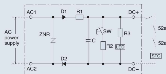
Fig. 95 Circuit diagram (KF-100E).
