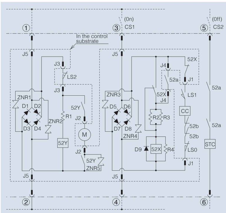
Fig. 100 Basic control circuit diagram.
