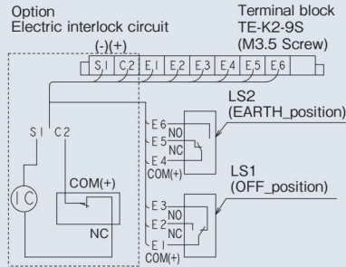
Connection diagram. (This connection diagram shows ES OFF position)
